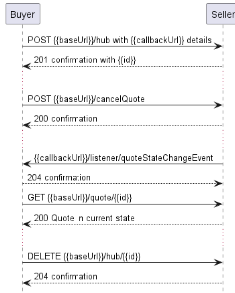
Figure 21 Use case 4, 5: Cancel or Decline Quote by Quote Identifier
